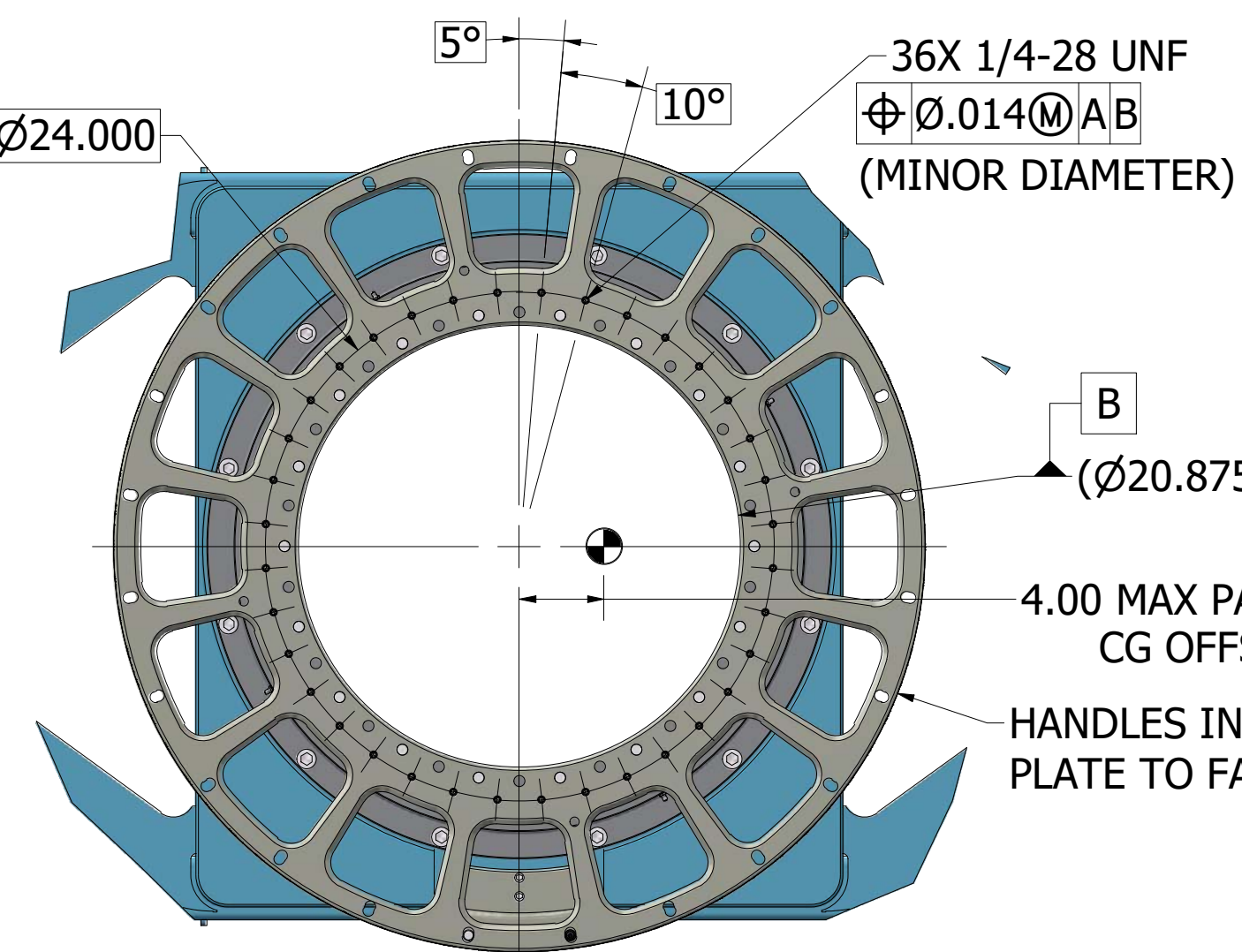
DETAIL G SCALE 1 : 8 INTERFACE HOLE PATTERN (STANDARD 24" ESPA GRANDE HOLE PATTERN)
