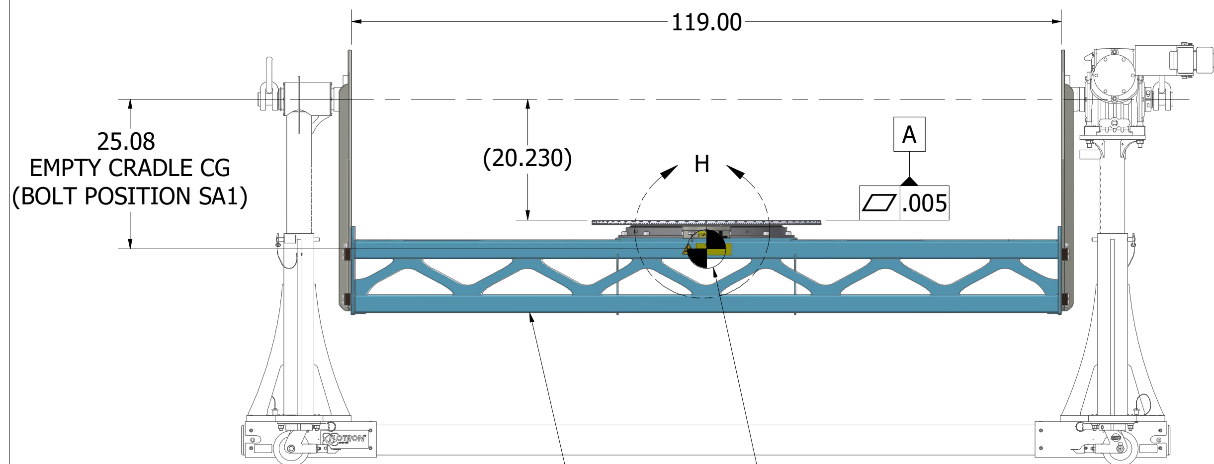
UNLOADED CRADLE CG @ BOLT POSITION 1 APPROXIMATE EMPTY CRADLE WEIGHT: 665 LBS
